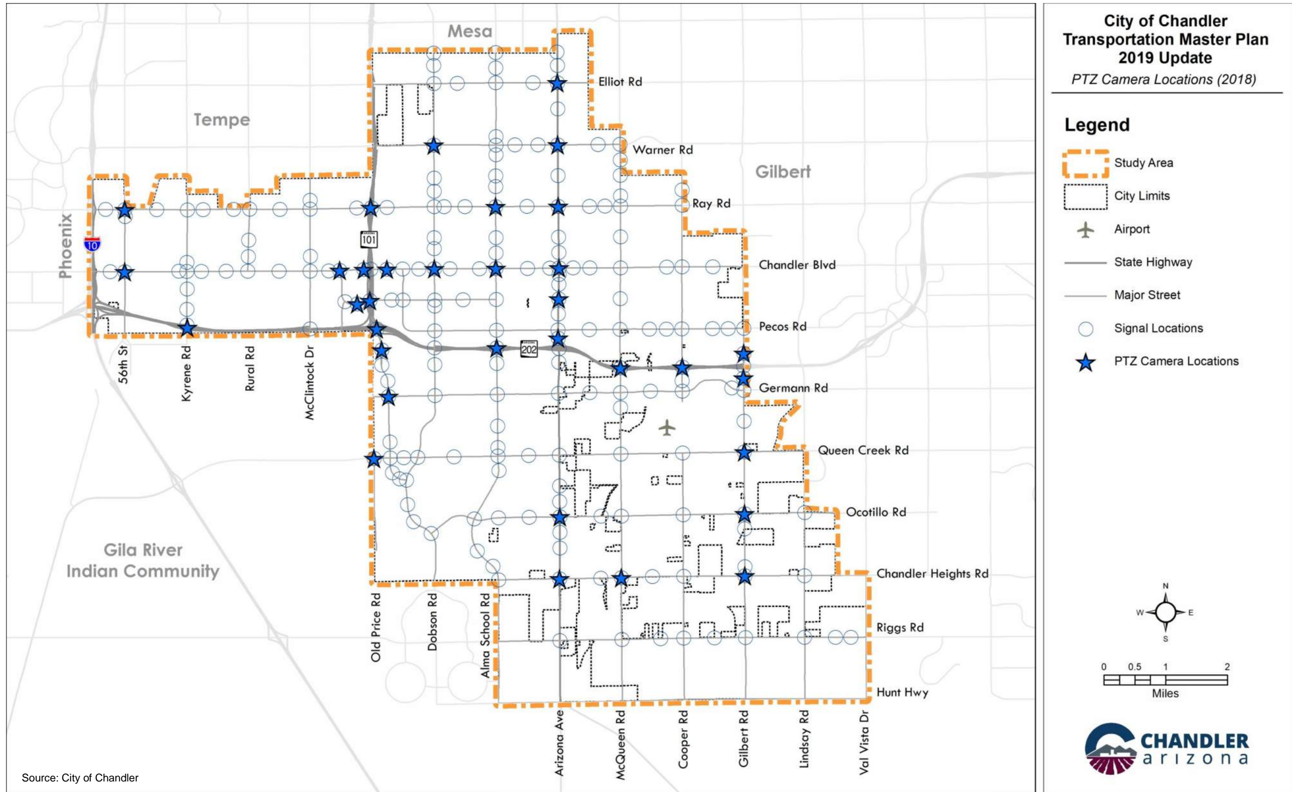
Figure 4-13. Intersections with Pan-Tilt-Zoom CCTV Cameras
